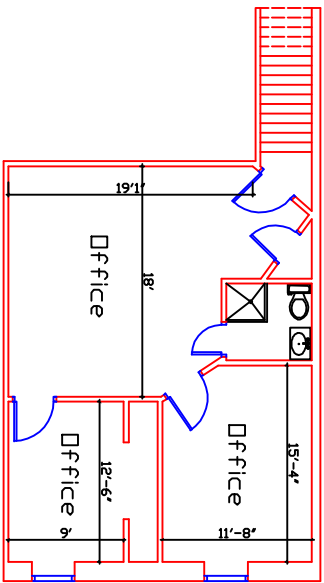
SECOND FLOOR Area : 812 Sq.Ft
